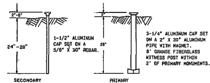
TYPICAL MONUMENT SETTINGS
